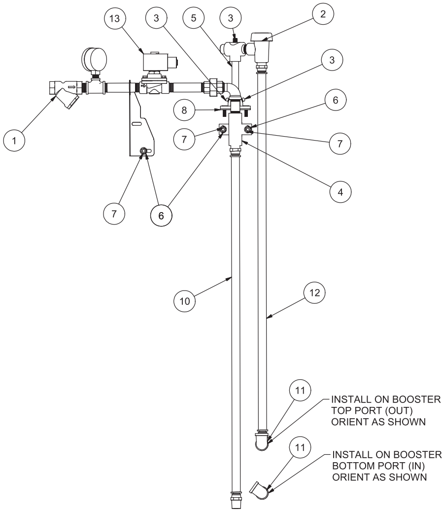
Back View
